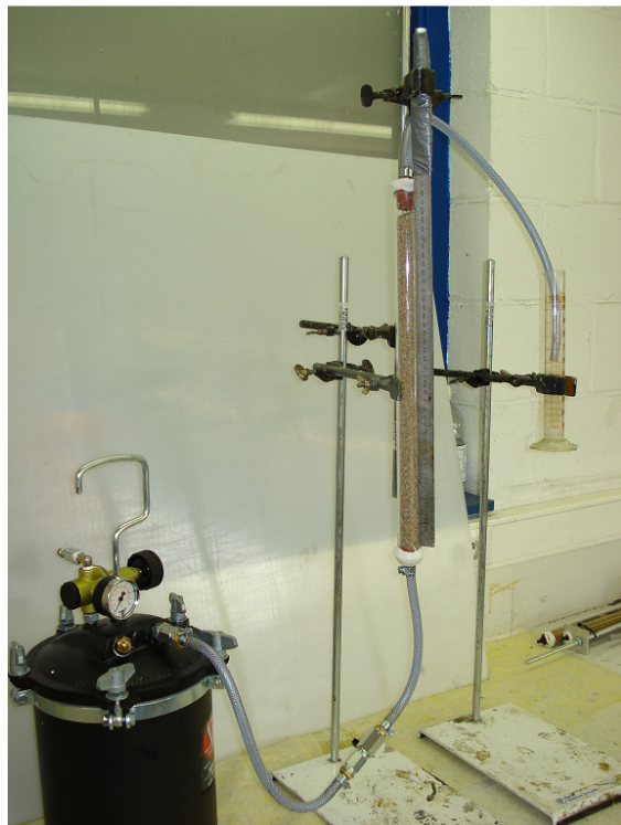
Photo 2 : Total test configuration before injection and before humidification.
